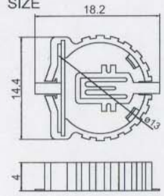
FOR CR1220 BATTERY SIZE
