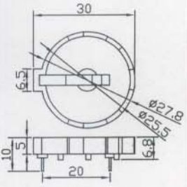
FOR CR2430 BATTERY SIZE
