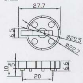
FOR CR2016 BATTERY SIZE
