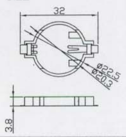
FOR CR2025 BATTERY SIZE
