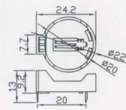
FOR CR2032 BATTERY SIZE
