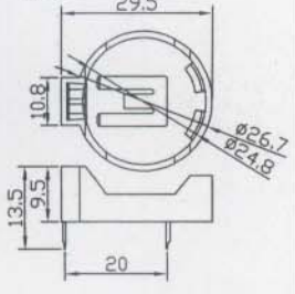
FOR CR2450 BATTERY SIZE
