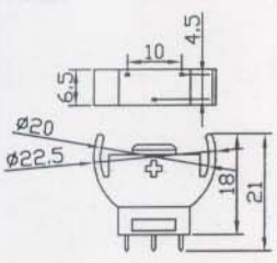
FOR CR2032 BATTERY SIZE
